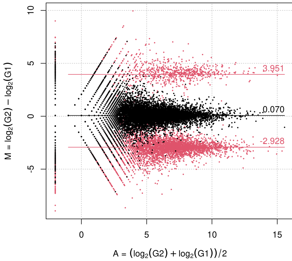
MA plot
