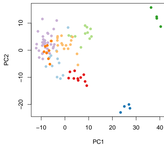
Figure 18: PCA plot for WT and FGF4-KO samples
