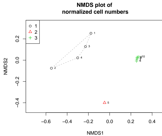
Figure 11: NMDS plot with groups
