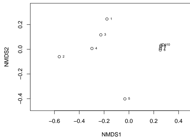
Figure 9: NMDS plot of normalized cell numbers using default parameters
