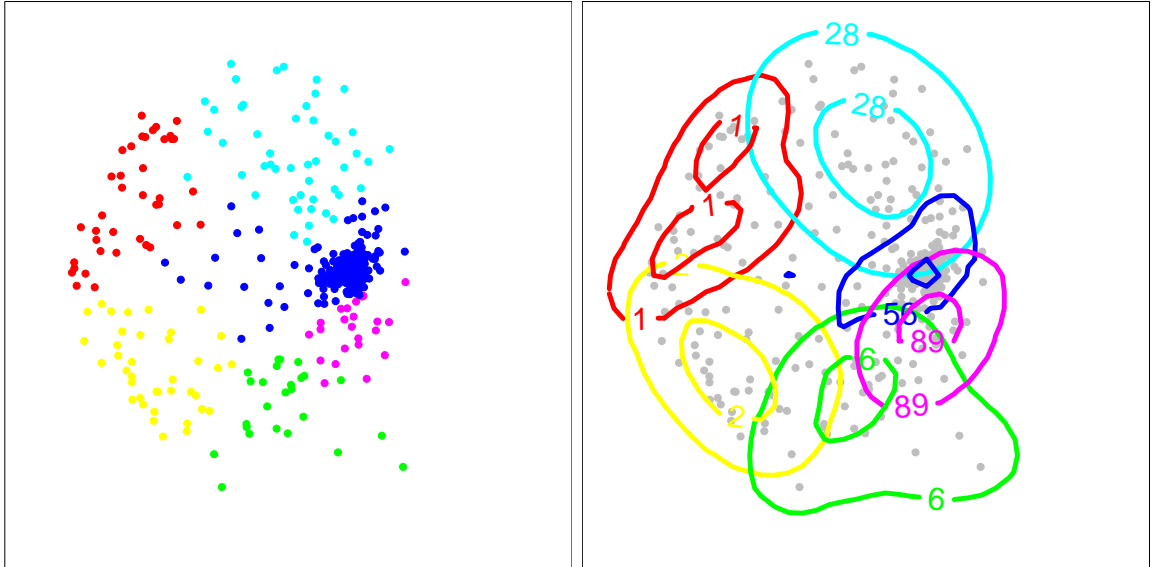
Figure 6: 2-dimensional MDS plot with \text{chromoGPS}^{\text{genes}} map and cluster identities indicated by point colors (left) and probabilistic contours drawn at 50 and 95 percent (right).
