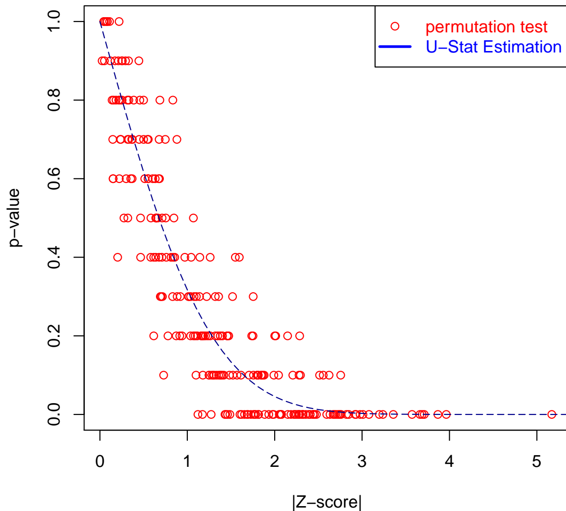
Figure 1: Comparing p-value from permutation test and U-statistic theory with only 10 permutations.
