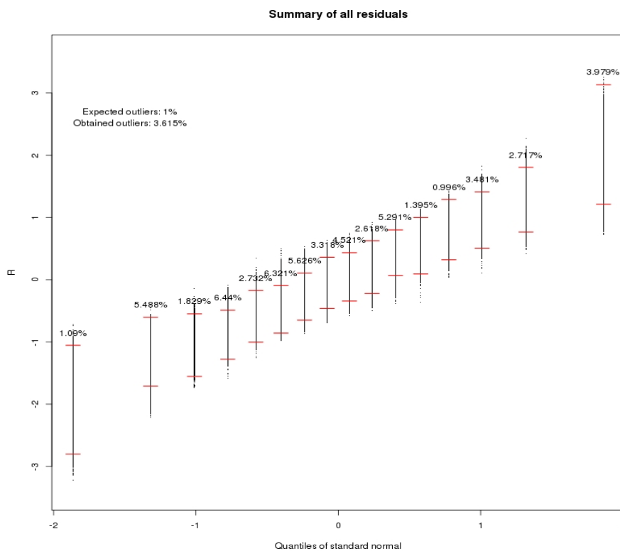
Figure 8: Assessment of whether the residuals are approximately normally distributed for a poor-quality data set
