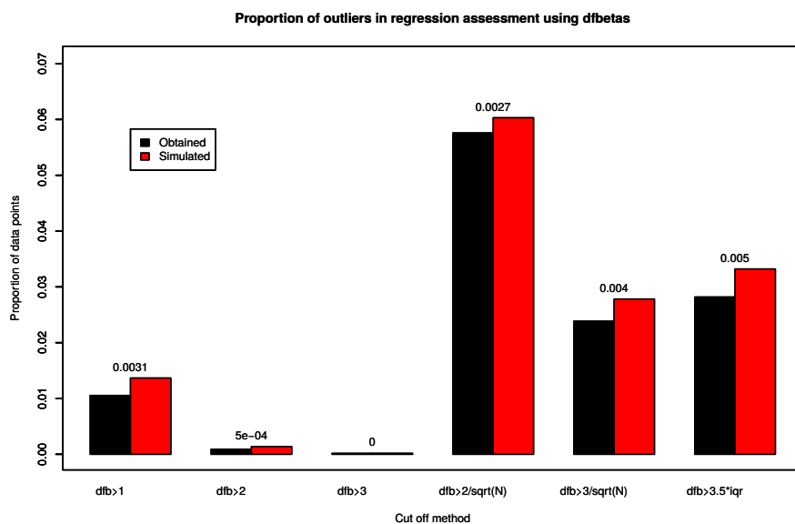
Figure 7: A bar graph showing the obtained and expected (based on a simulation) number of influential data points as judged by different thresholds for a poor-quality data set For each threshold the difference between the obtained and the simulated frequency of outliers is shown. Notice that fewer influential data points as compared what is expected by chance is observed.
