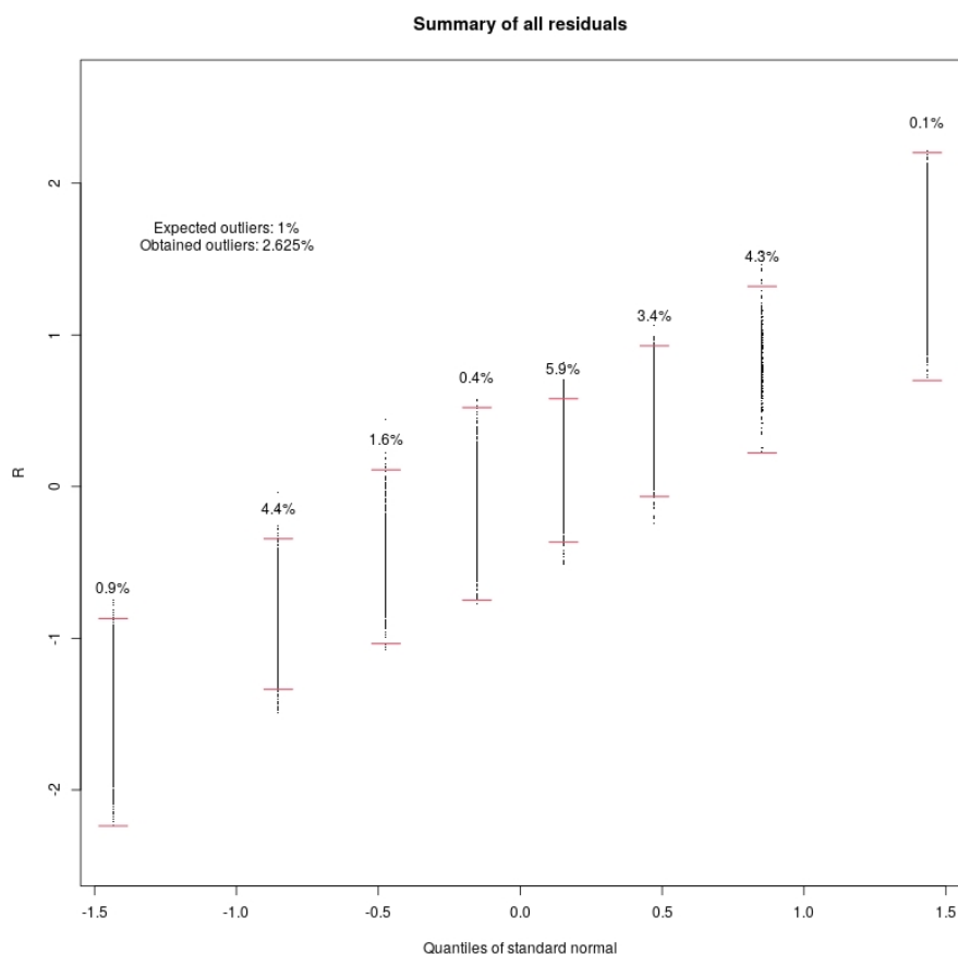
Figure 5: Assessment of whether the residuals are approximately normally distributed Shown is the output from all features using the anota2seqResidOutlierTest function. The Q-Q plot for the features is compared to the outer limits of a set of Q-Q plots generated by sampling from the normal distribution. The obtained and expected percentage of outliers is indicated at each rank position and combined.
