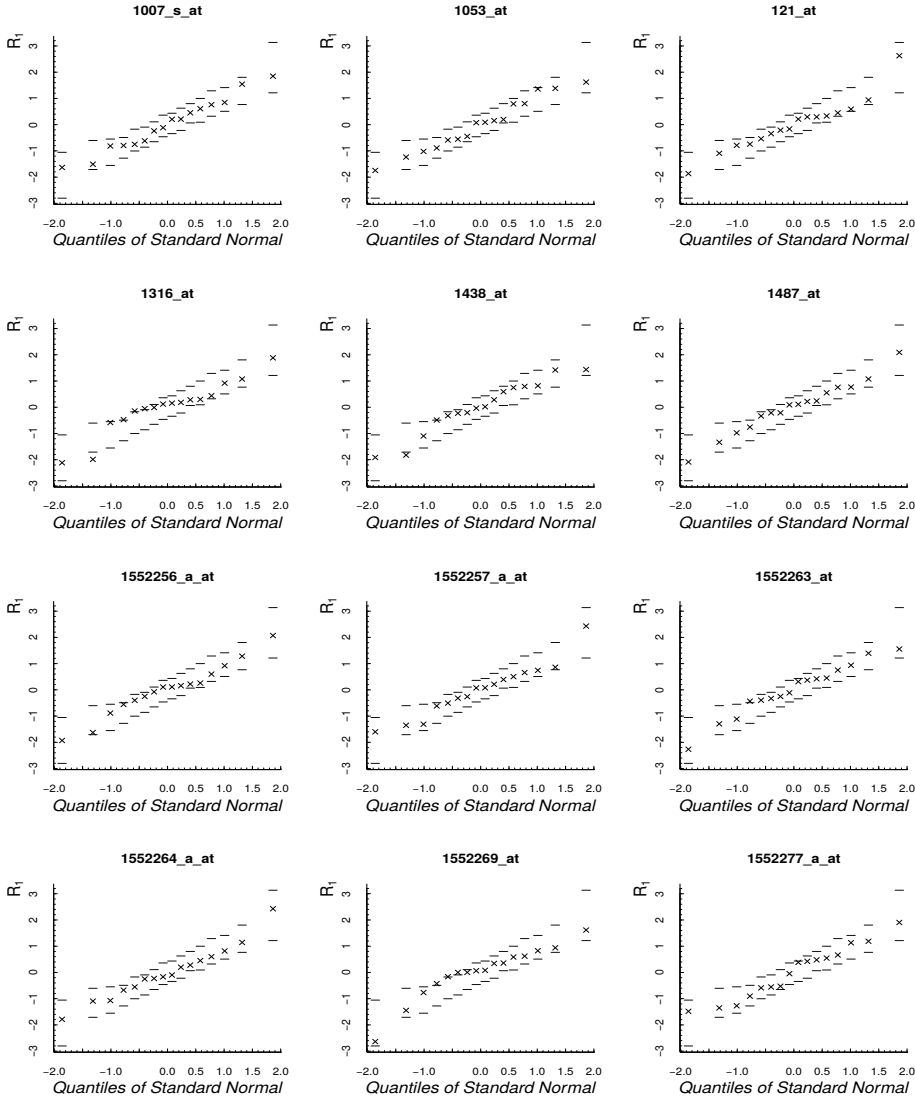
Figure 9: Assessment of whether the residuals are approximately normally distributed for a poor-quality data set Shown is the output from the single feature alternative within anota2seqResidOutlierTest . The Q-Q plot for the feature is compared to the outer limits of a set of Q-Q plots generated by sampling from the normal distribution. Notice, that residuals from several individual features (residual from each samples is indicated with an "x") show a non-linear pattern.
