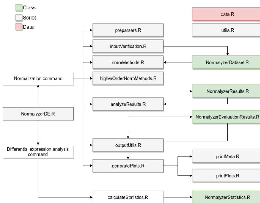
Figure 1: NormalizerDE schematics
