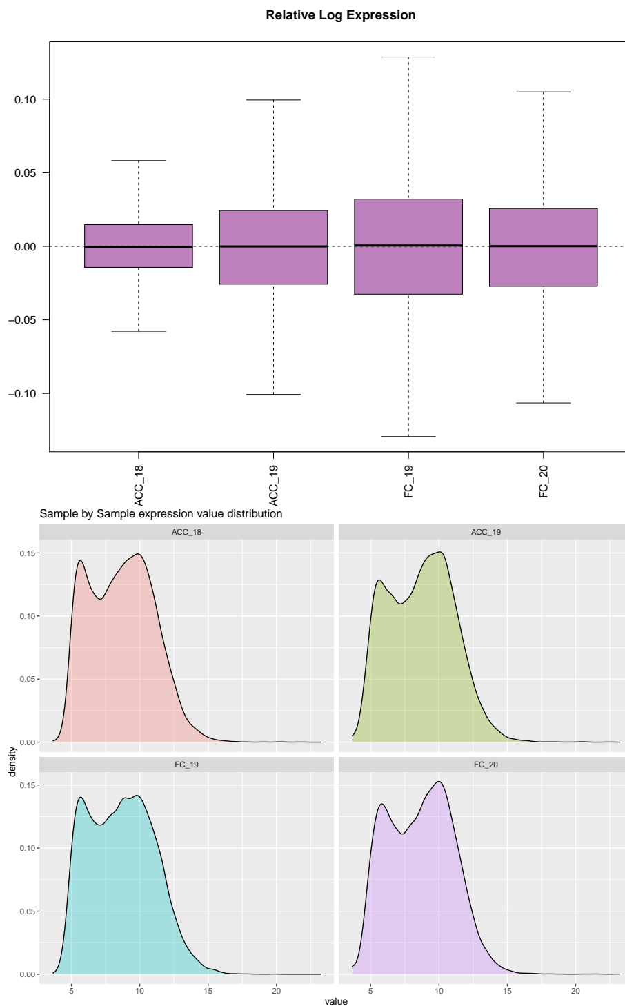
Figure 17: RLE and Gene Expression distribution after normalization
