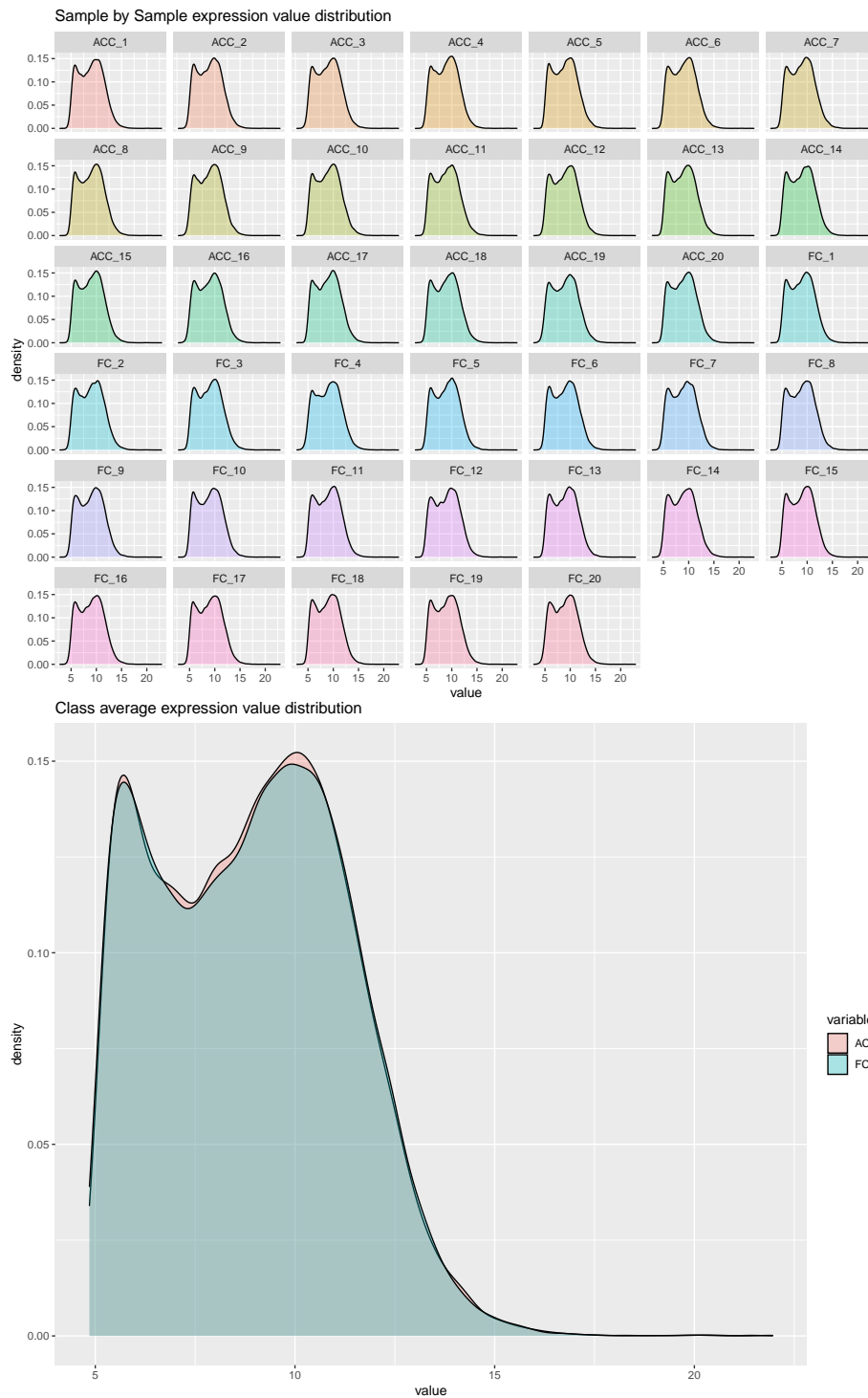
Figure 10: Gene Expression distribution
