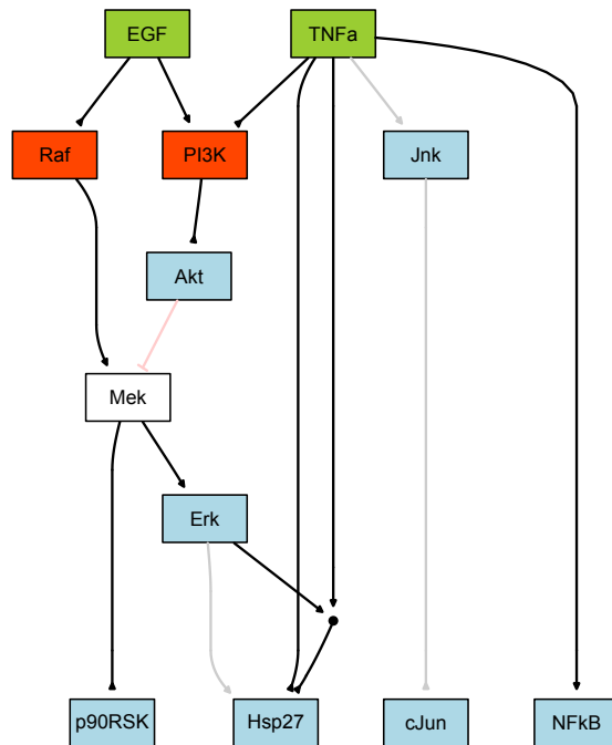
Figure 13: Results of the lpBinaryT1 function on the Toy Model example - solution 3
