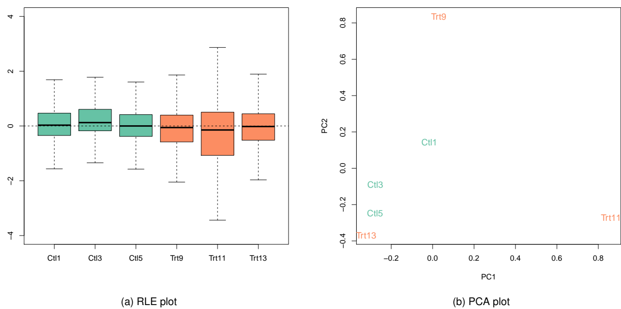
Figure 2: Upper-quartile normalization.
