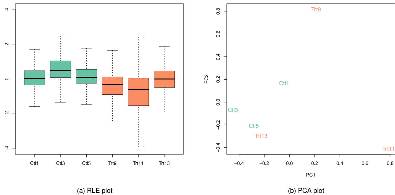
Figure 1: No normalization.
